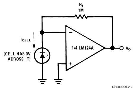
Photo Voltaic-Cell Amplifier
