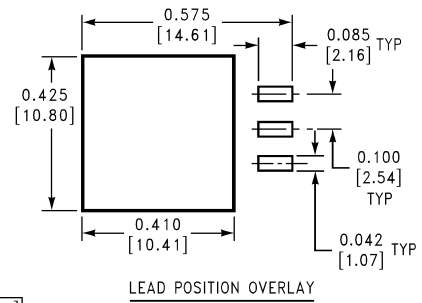
LEAD POSITION OVERLAY
